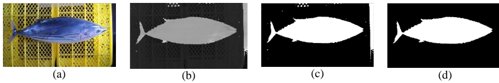
Gambar 3. Proses Segmentasi Citra (a) Citra Asli; (b) Citra Hue; (c) Citra Biner Ber-noise; (d) Hasil Segmentasi
